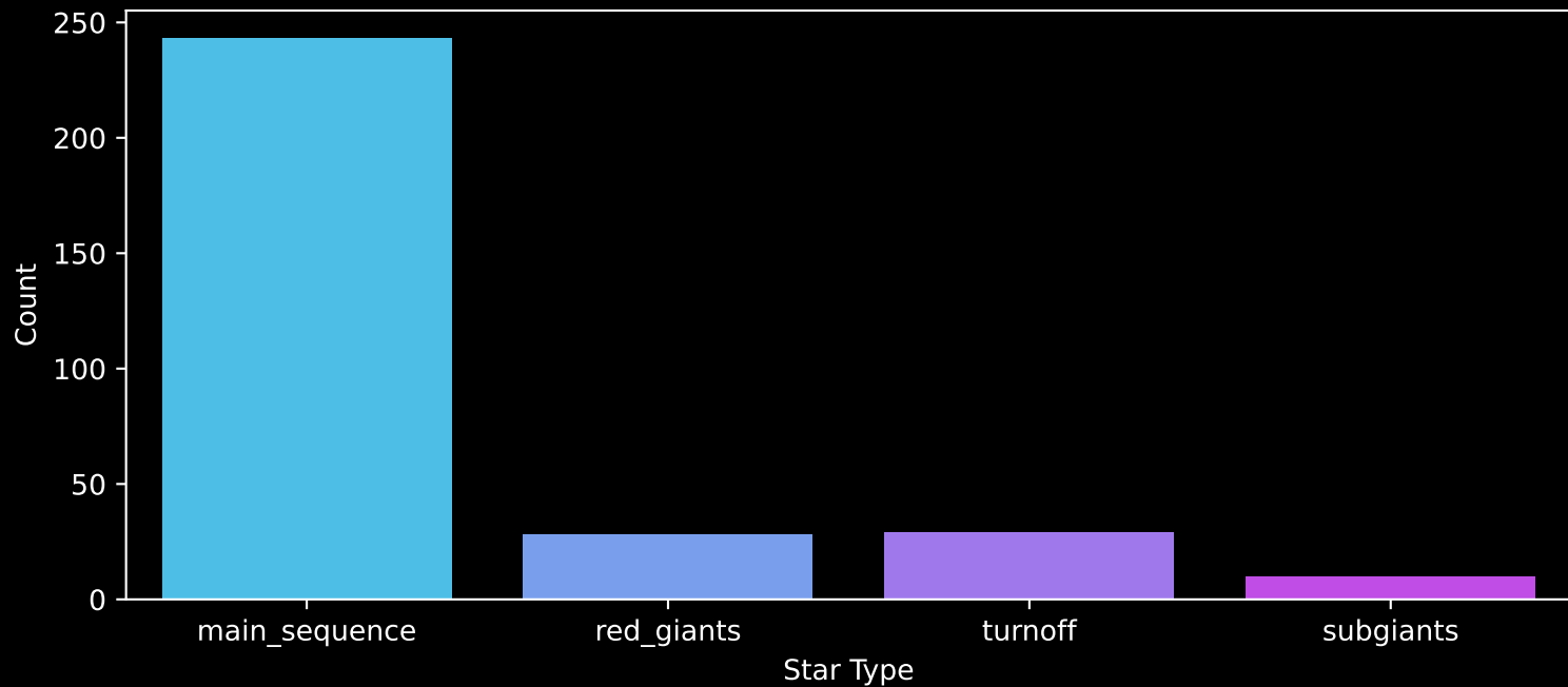
APOGEE DR17 Field: [SGRT-2] Count plot of Star Type
