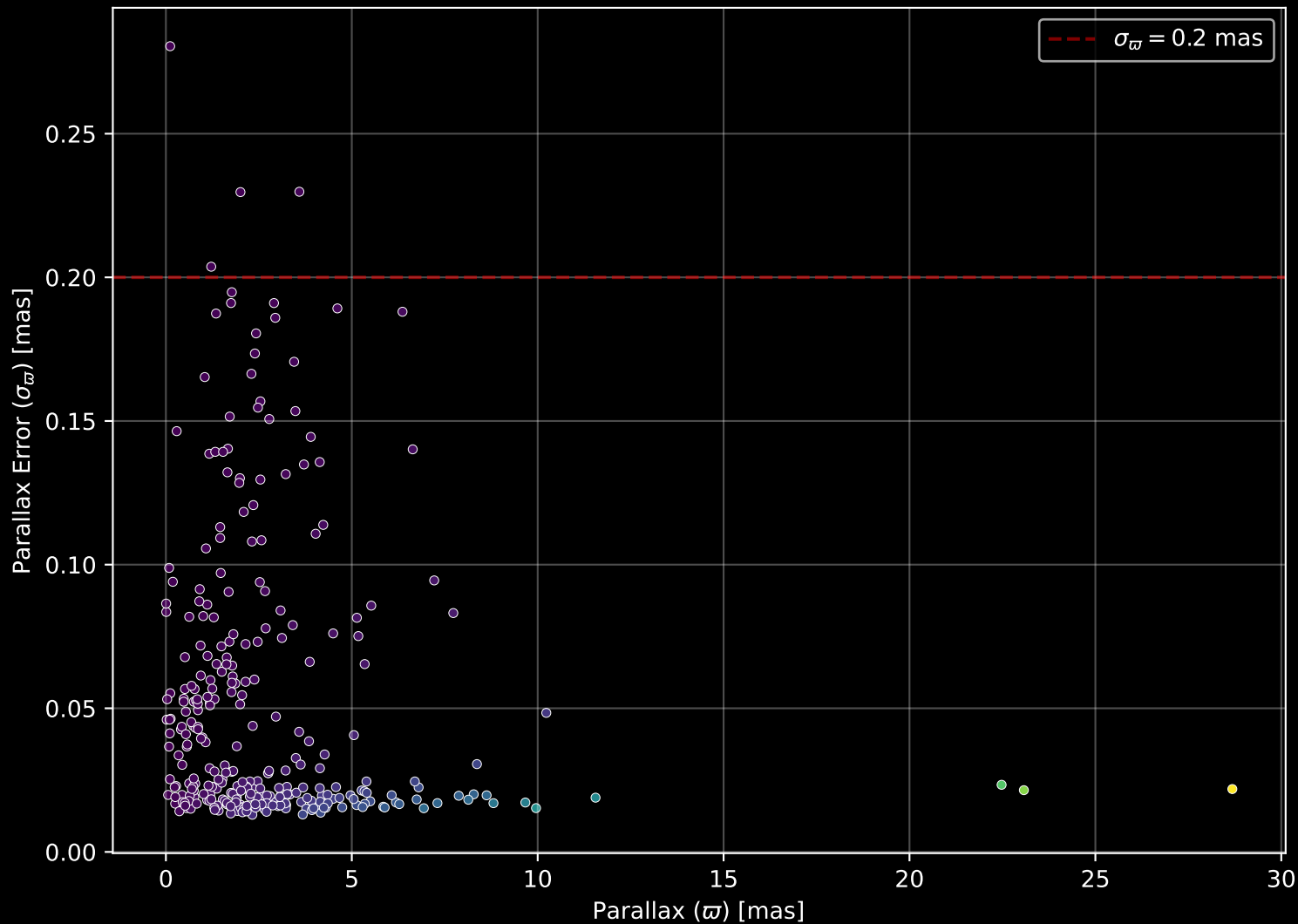
APOGEE DR17 Field: [SGRT-2] Parallax Quality (n= 310)
