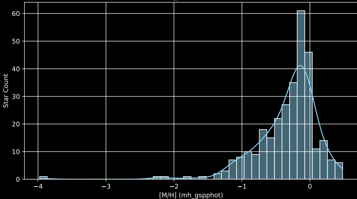
APOGEE DR17 Field: [SGRT-2 [M/H] (mh_gspphot) (n= 306)
