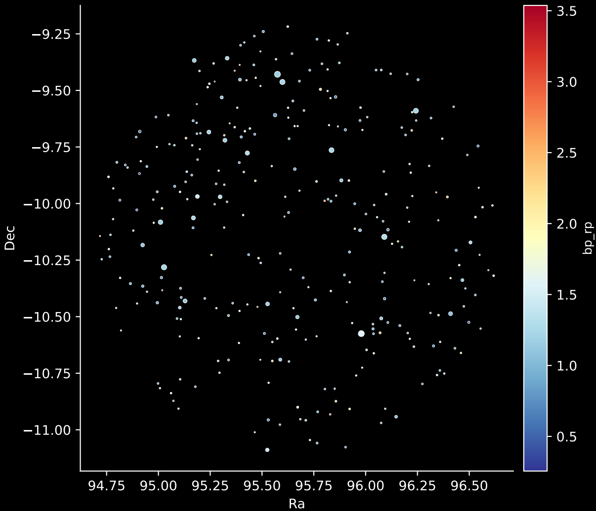
APOGEE DR17 Field: [SGRT-2] Stars: 310
