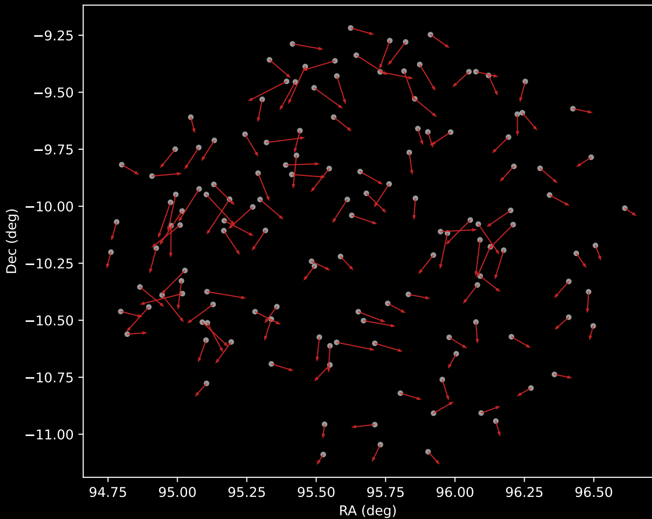
APOGEE DR17 Cluster 6 Proper Motion Vectors (n=138)
