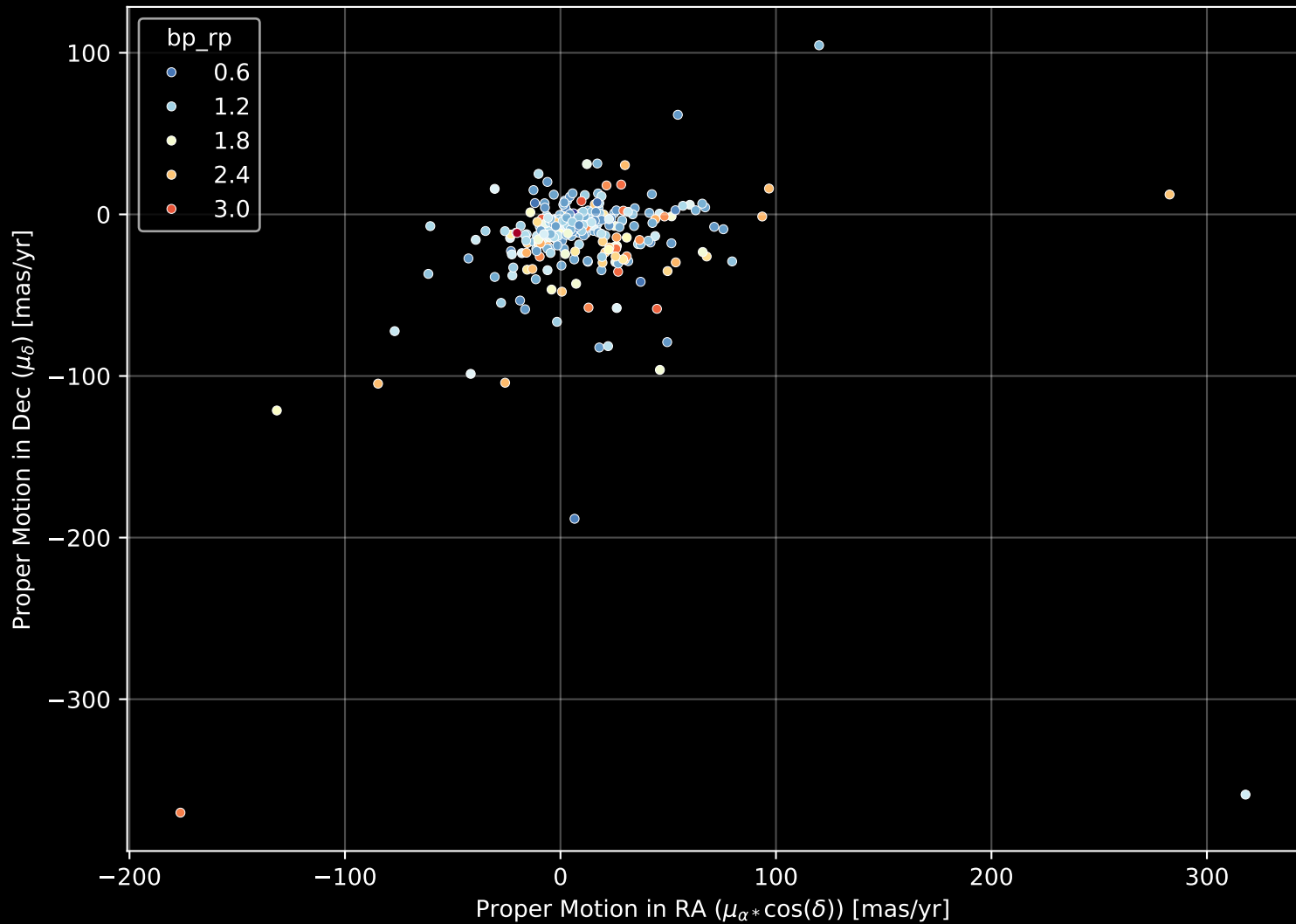
APOGEE DR17 Field: [SGRT-2] Proper Motion Diagram (n= 310)
