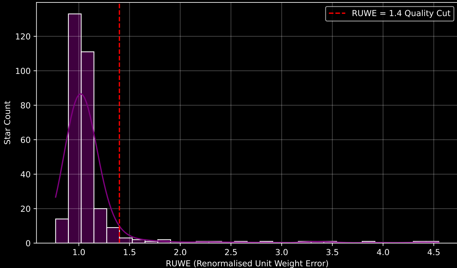
GAPOGEE DR17 Field [SGRT-2] RUWE Distribution (n= 305)
