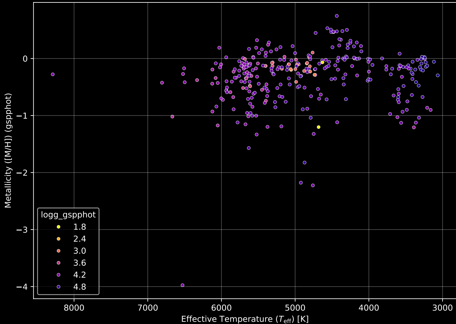
APOGEE DR17 Field: [SGRT-2] Stellar Population Parameters (n= 310)
